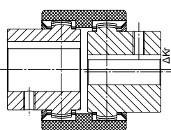
radial misalignment
