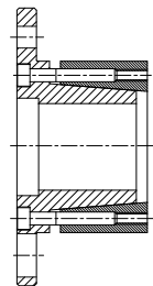
Shrink disc hub I
