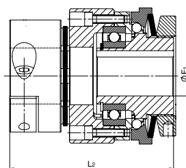
Bore and keyway execution / GSM
